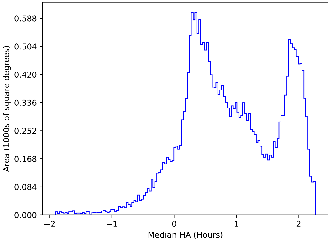
internal_u_expt45_nscale1.0v3.4_10yrs All sky all bands: Median HA
