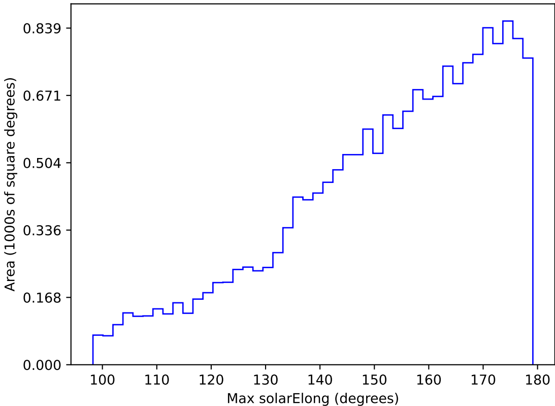
internal_u_expt45_nscale1.0v3.4_10yrs WFD u band: Max solarElong
