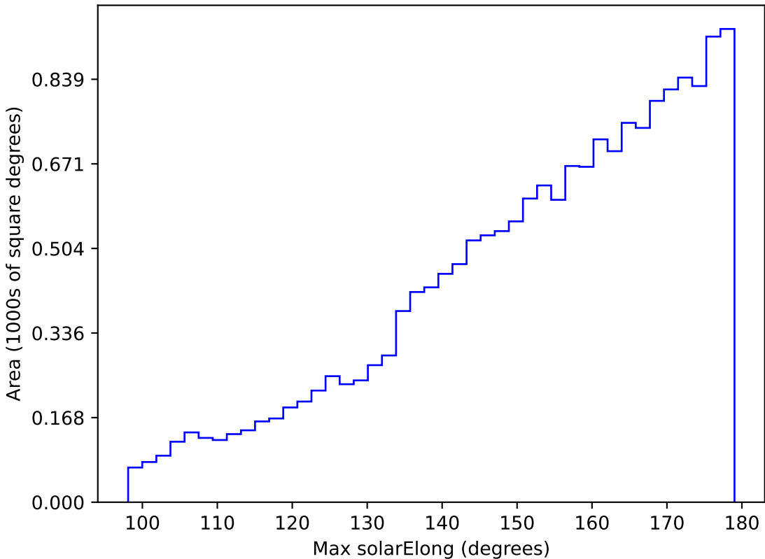
internal_u_expt45_nscale1.0v3.4_10yrs WFD g band: Max solarElong
