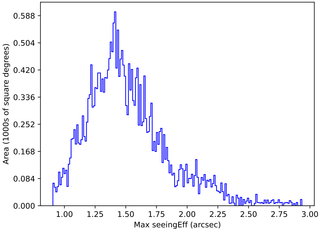
internal_u_expt45_nscale1.0v3.4_10yrs Yr 1 z band: Max seeingEff
