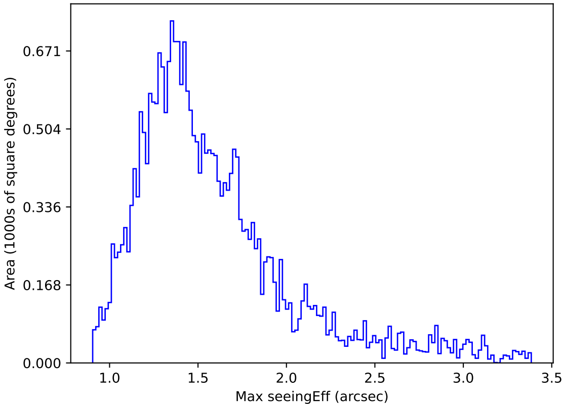
internal_u_expt45_nscale1.0v3.4_10yrs Yr 1 i band: Max seeingEff
