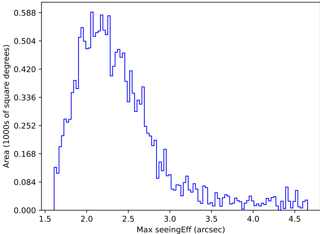
internal_u_expt45_nscale1.0v3.4_10yrs WFD y band: Max seeingEff
