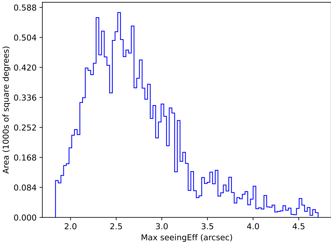
internal_u_expt45_nscale1.0v3.4_10yrs WFD r band: Max seeingEff
