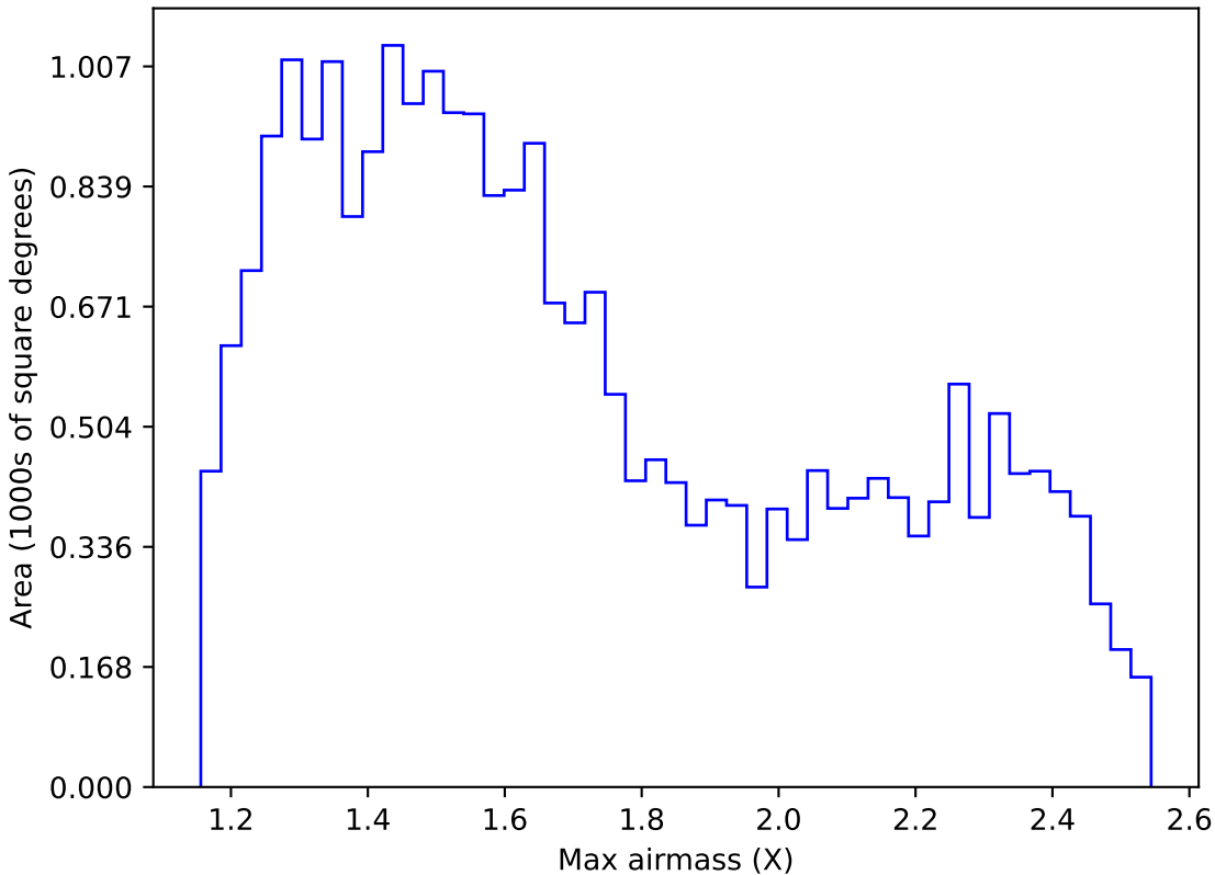
internal_u_expt45_nscale1.0v3.4_10yrs Yr 1 r band: Max airmass
