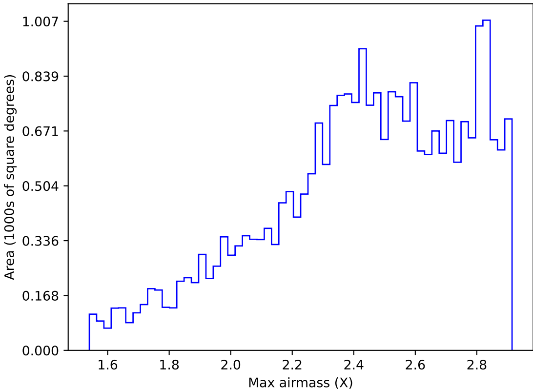
internal_u_expt45_nscale1.0v3.4_10yrs All sky i band: Max airmass
