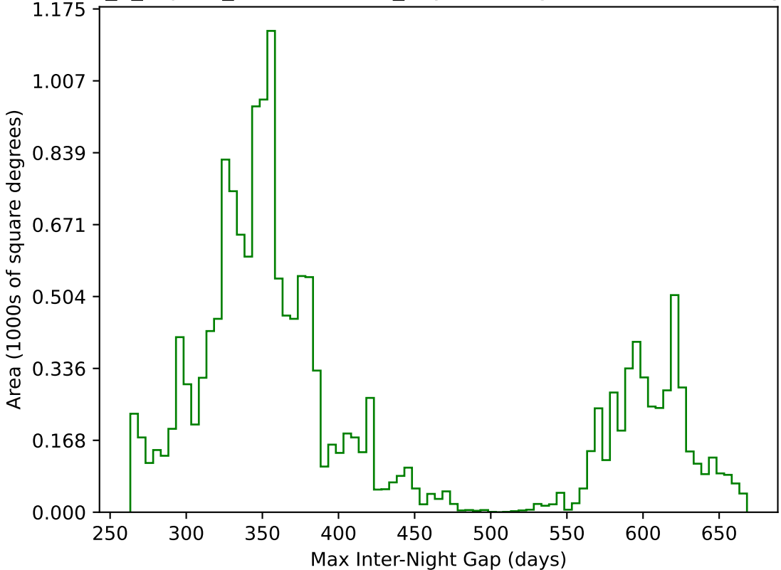
internal_u_expt45_nscale1.0v3.4_10yrs WFD g band: Max Inter-Night Gap
