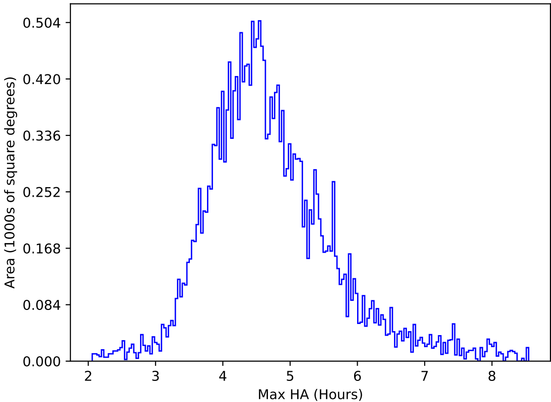
internal_u_expt45_nscale1.0v3.4_10yrs All sky y band: Max HA
