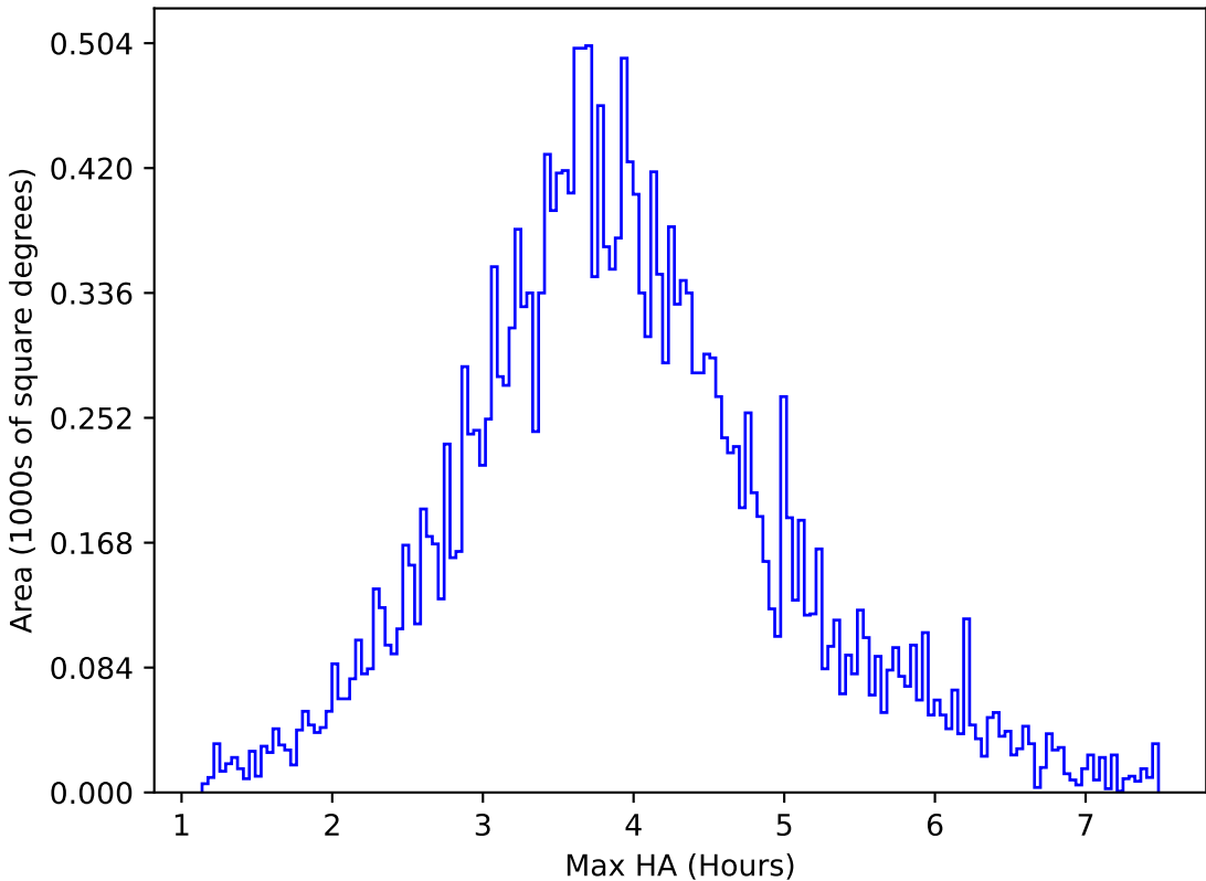
internal_u_expt45_nscale1.0v3.4_10yrs All sky u band: Max HA
