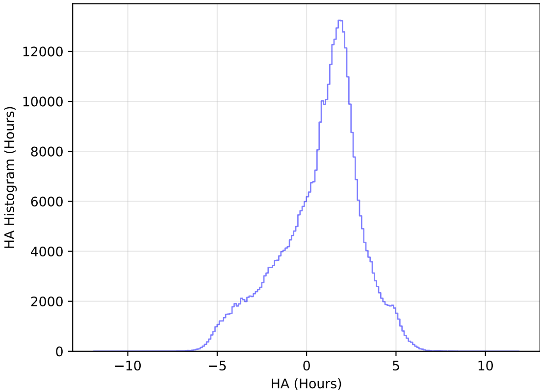
internal_u_expt45_nscale1.0v3.4_10yrs WFD z band: HA Histogram
