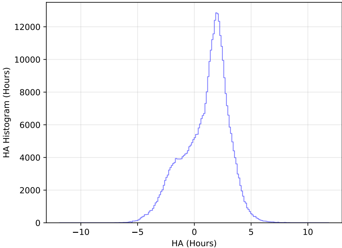
internal_u_expt45_nscale1.0v3.4_10yrs WFD y band: HA Histogram
