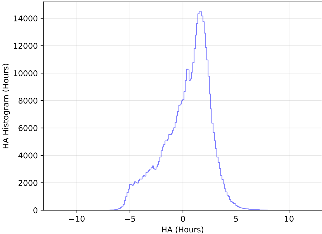
internal_u_expt45_nscale1.0v3.4_10yrs WFD r band: HA Histogram
