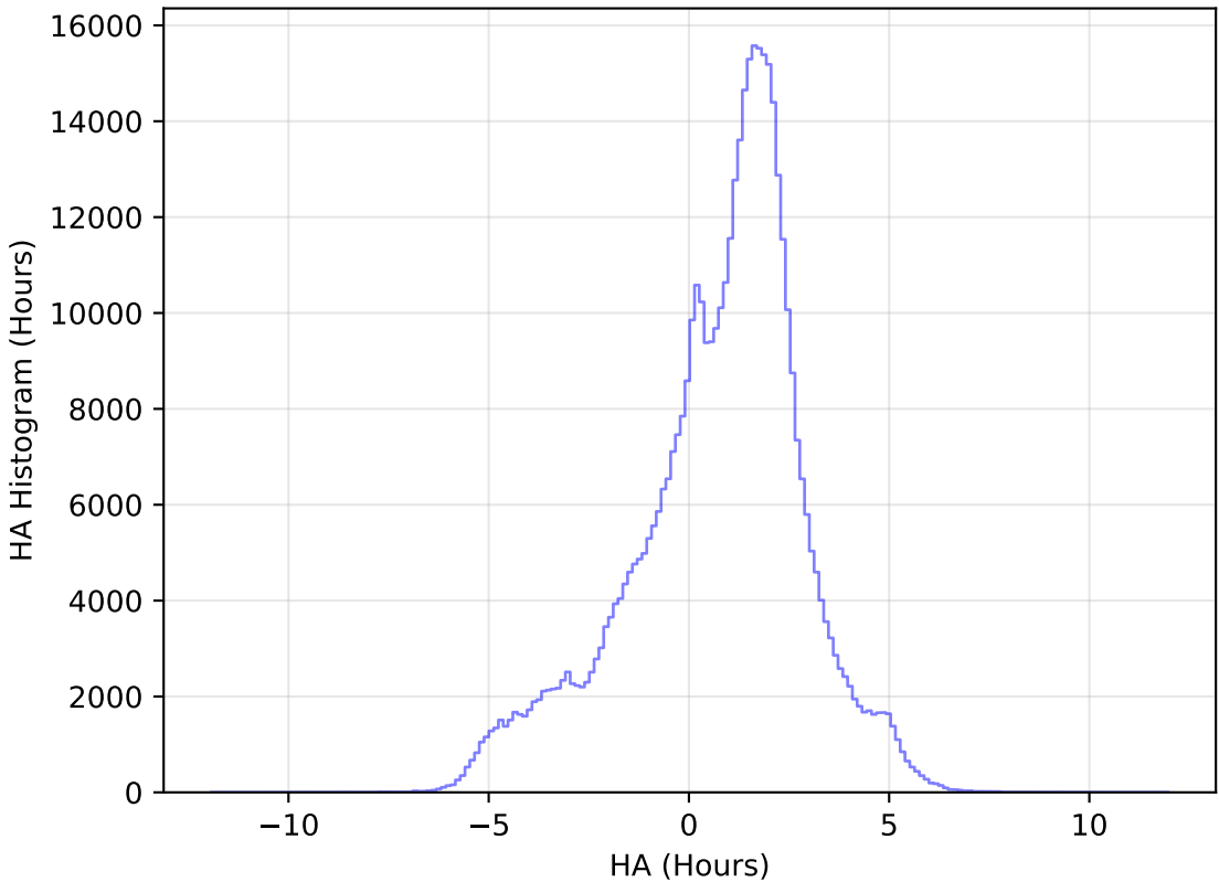
internal_u_expt45_nscale1.0v3.4_10yrs WFD i band: HA Histogram
