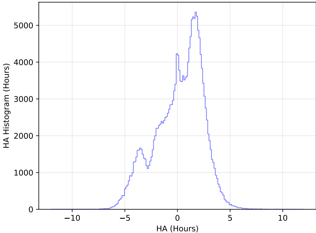
internal_u_expt45_nscale1.0v3.4_10yrs WFD g band: HA Histogram
