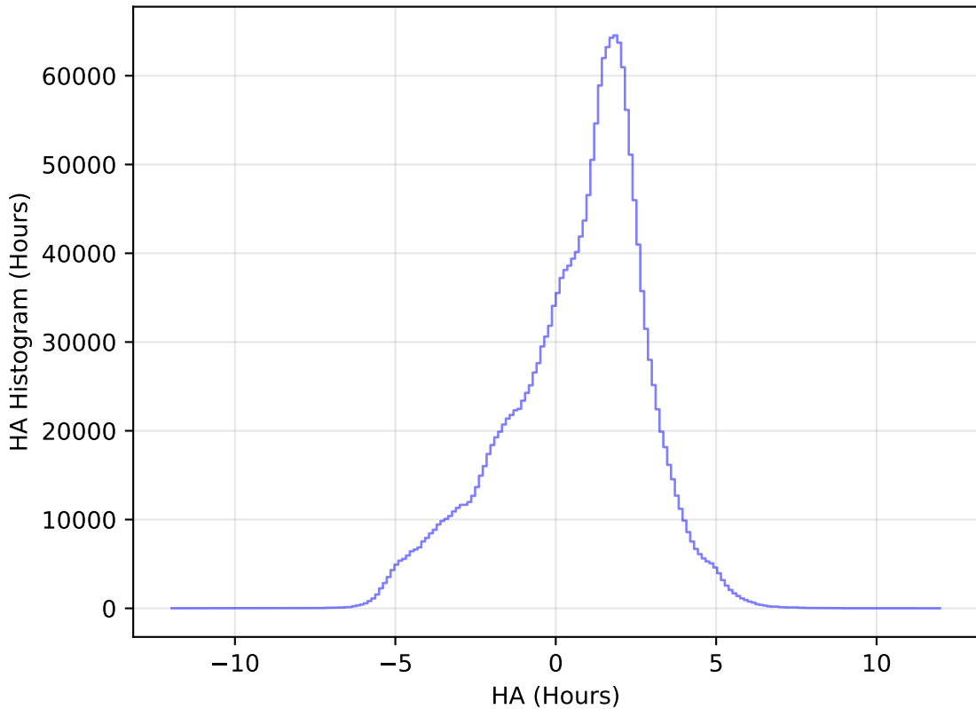
internal_u_expt45_nscale1.0v3.4_10yrs WFD all bands: HA Histogram
