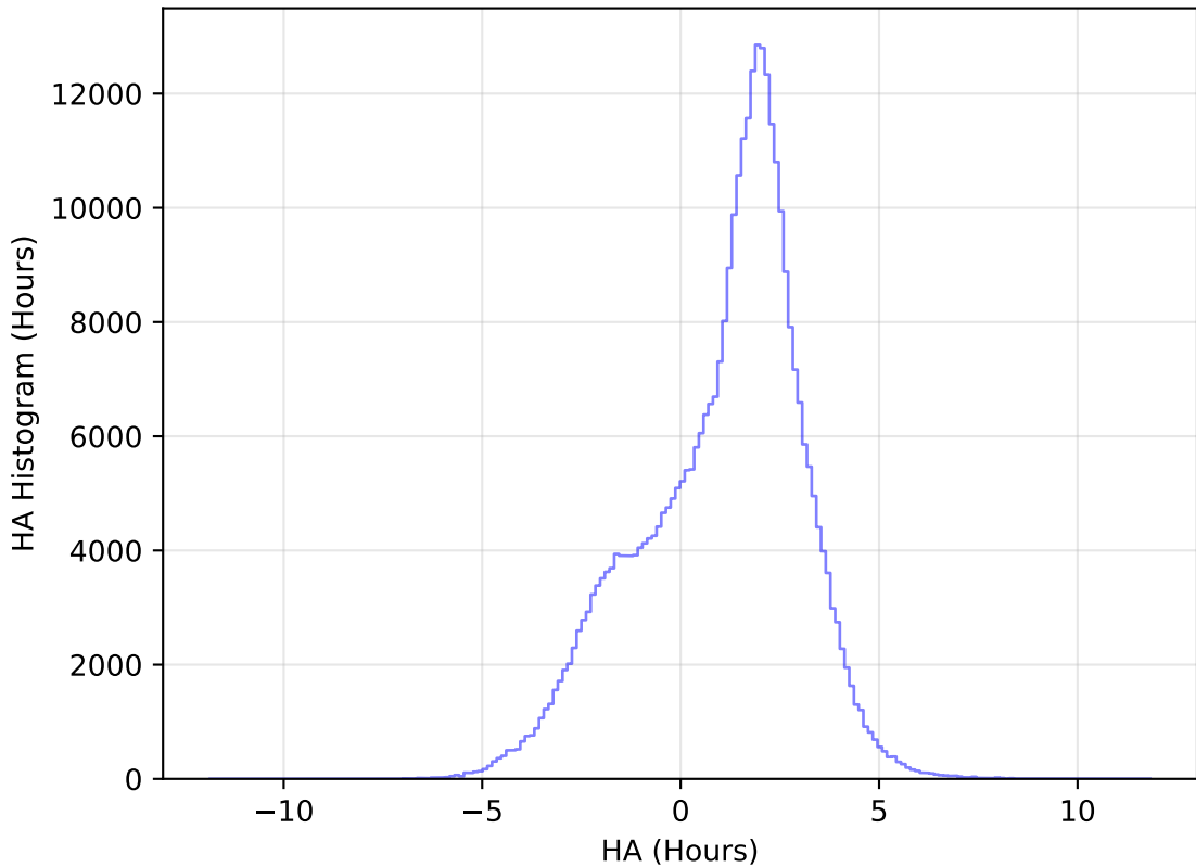
internal_u_expt45_nscale1.0v3.4_10yrs All sky y band: HA Histogram
