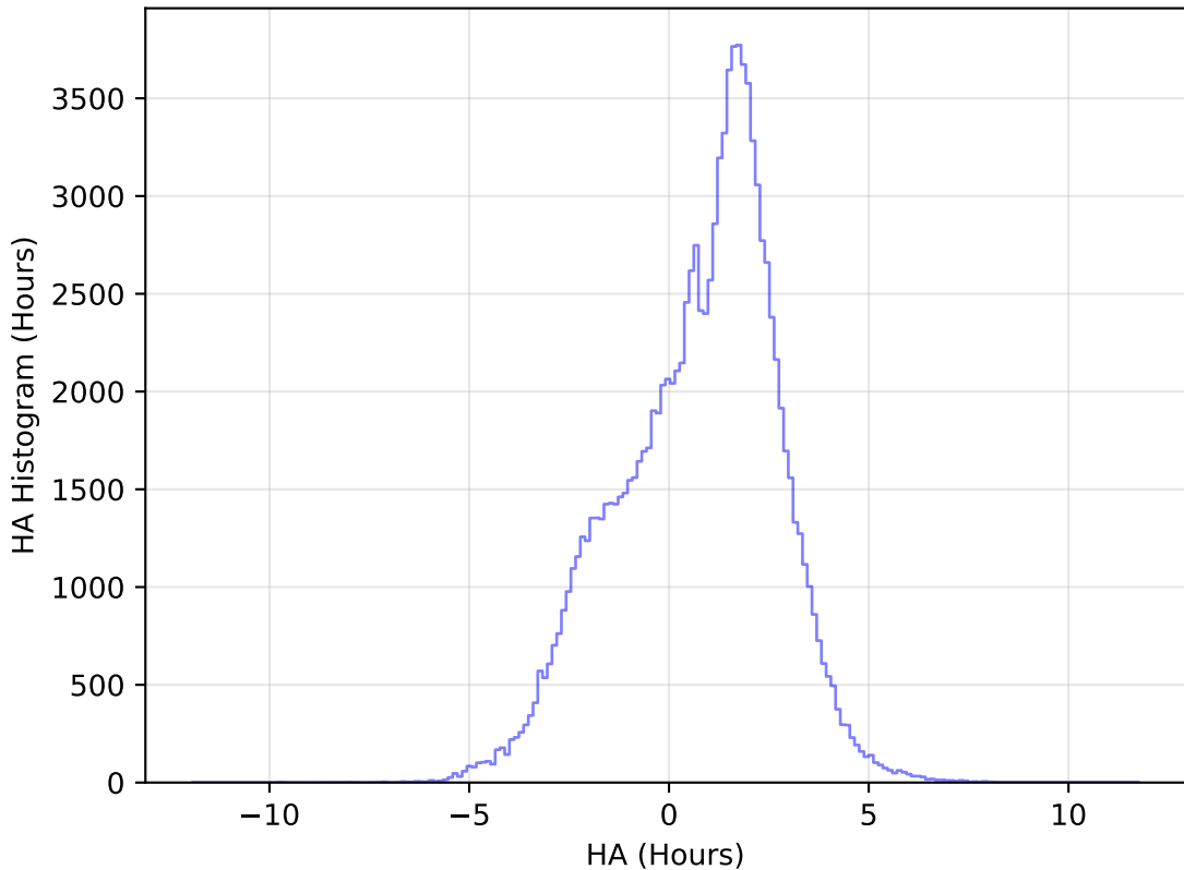
internal_u_expt45_nscale1.0v3.4_10yrs All sky u band: HA Histogram
