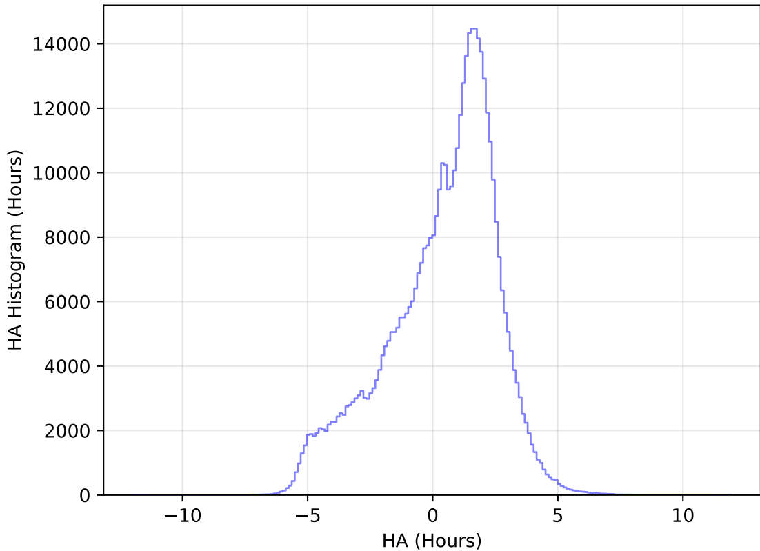
internal_u_expt45_nscale1.0v3.4_10yrs All sky r band: HA Histogram
