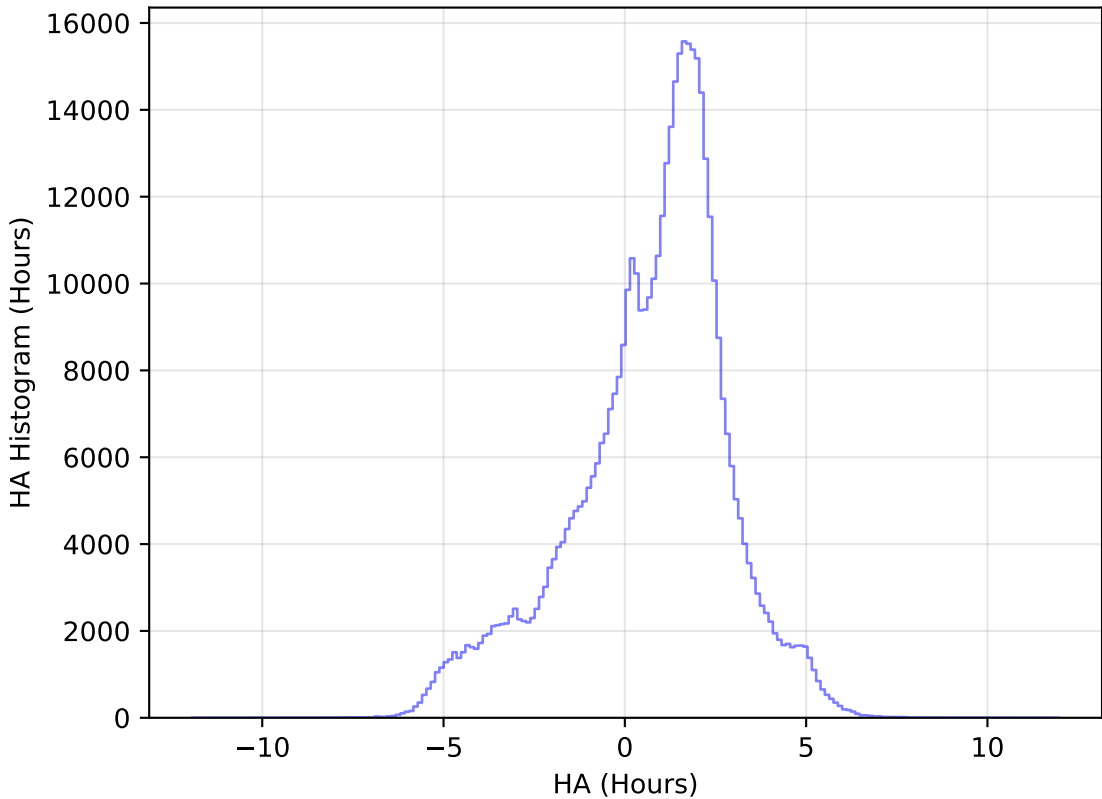
internal_u_expt45_nscale1.0v3.4_10yrs All sky i band: HA Histogram
