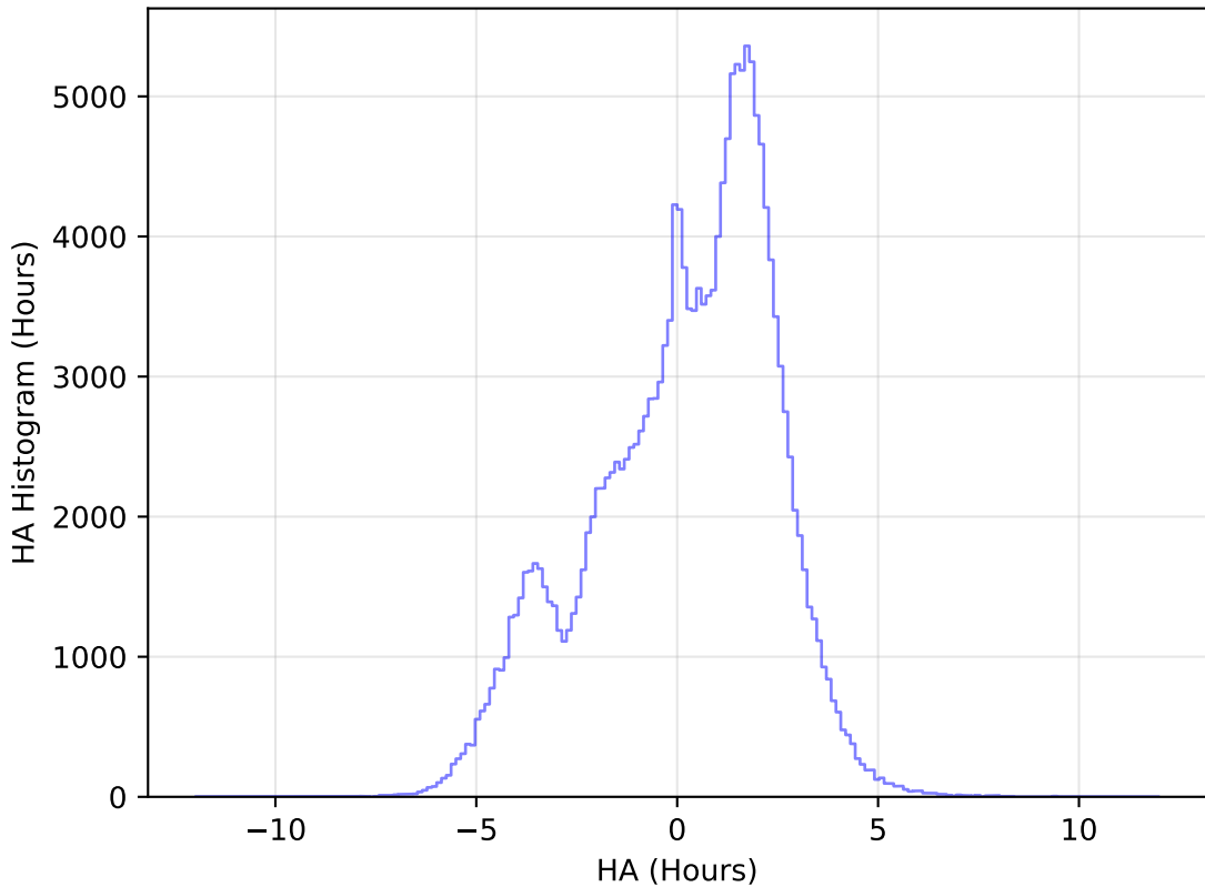
internal_u_expt45_nscale1.0v3.4_10yrs All sky g band: HA Histogram
