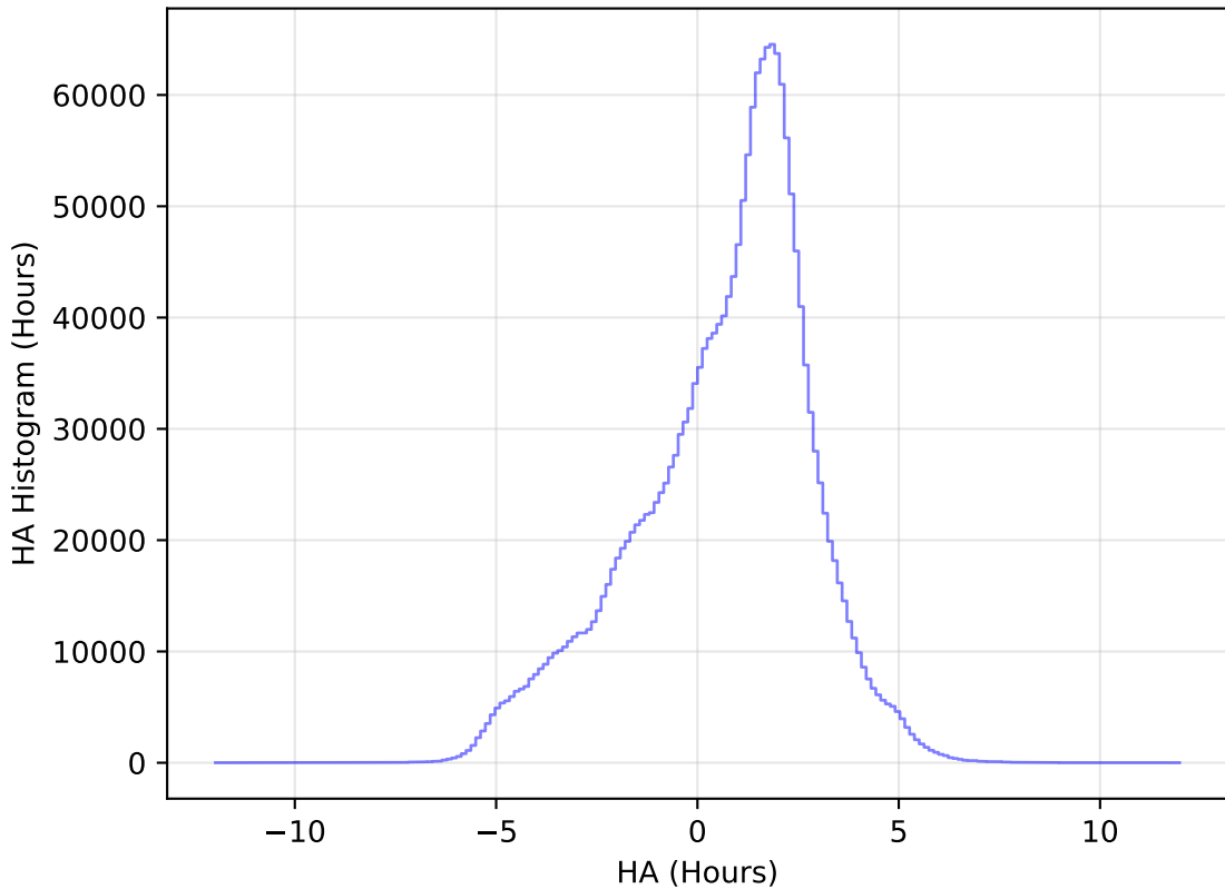
internal_u_expt45_nscale1.0v3.4_10yrs All sky all bands: HA Histogram
