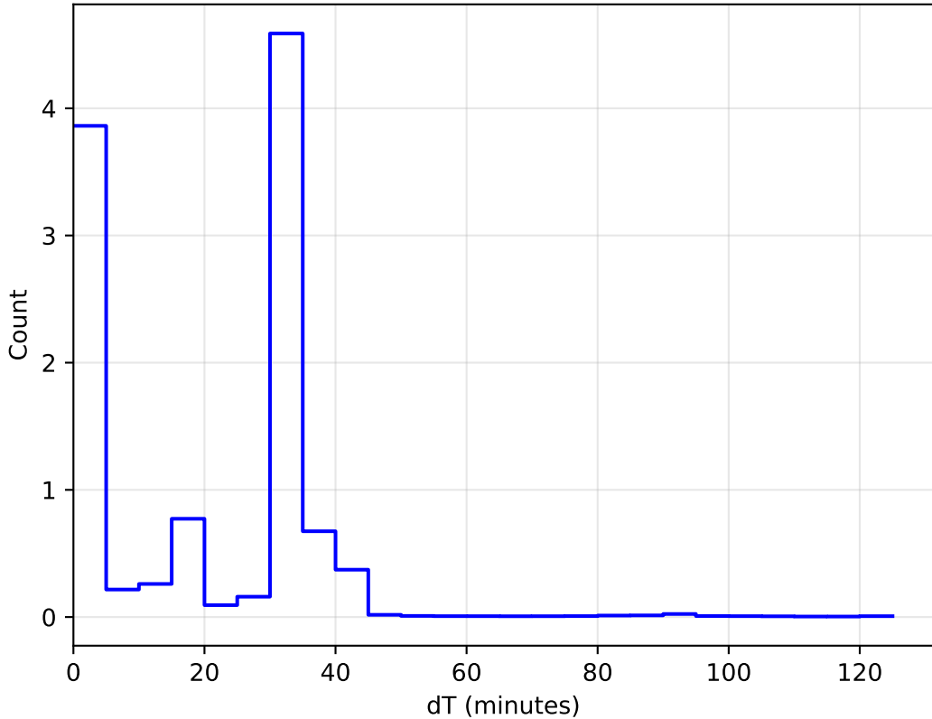
internal_u_expt45_nscale1.0v3.4_10yrs WFD: DeltaT Histogram
