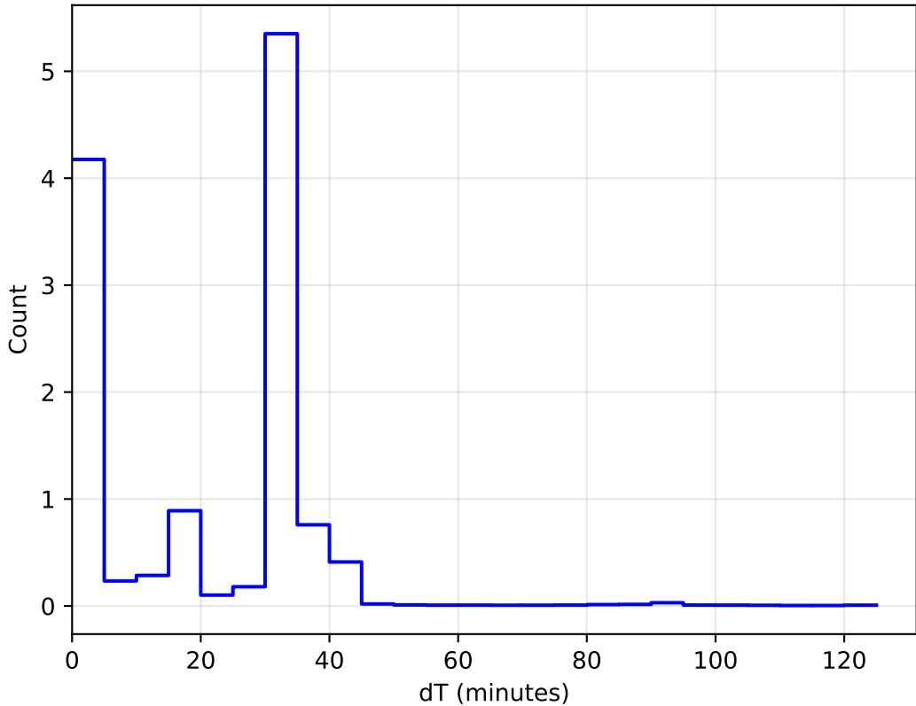
internal_u_expt45_nscale1.0v3.4_10yrs All sky: DeltaT Histogram
