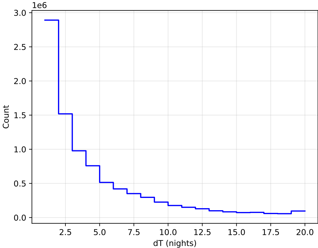
internal_u_expt45_nscale1.0v3.4_10yrs All sky all bands: DeltaNight Histogram
