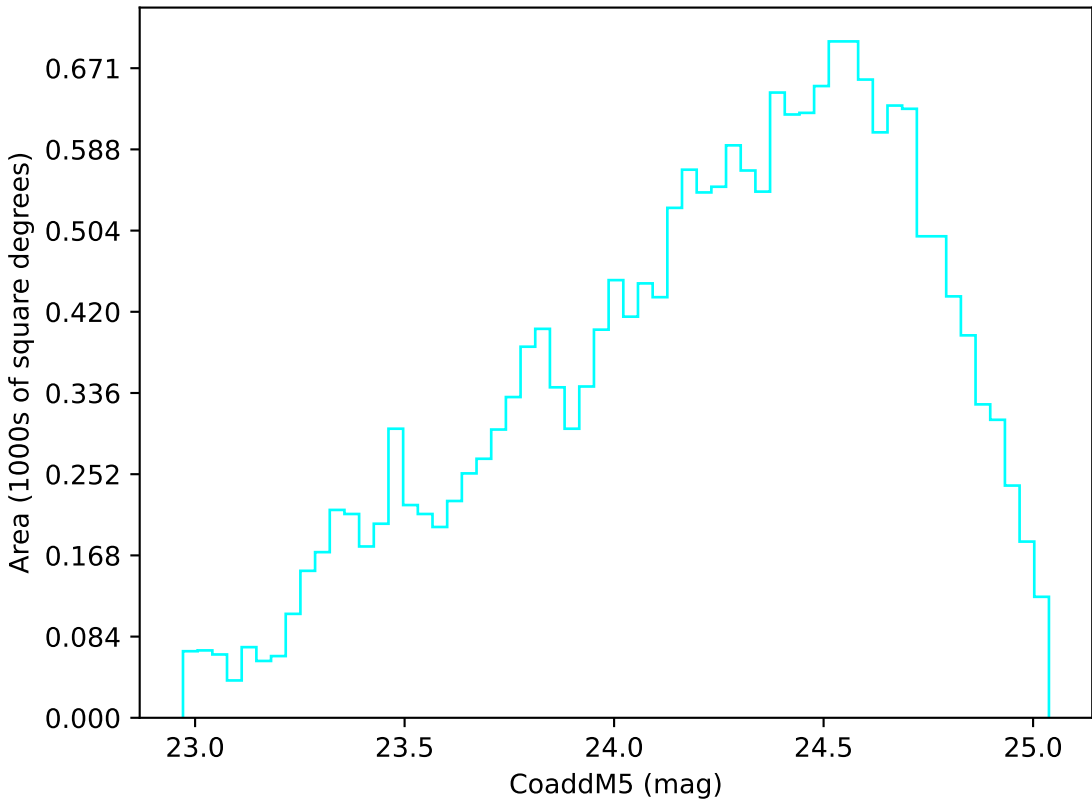
internal_u_expt45_nscale1.0v3.4_10yrs Yr 3-4 u band: CoaddM5
