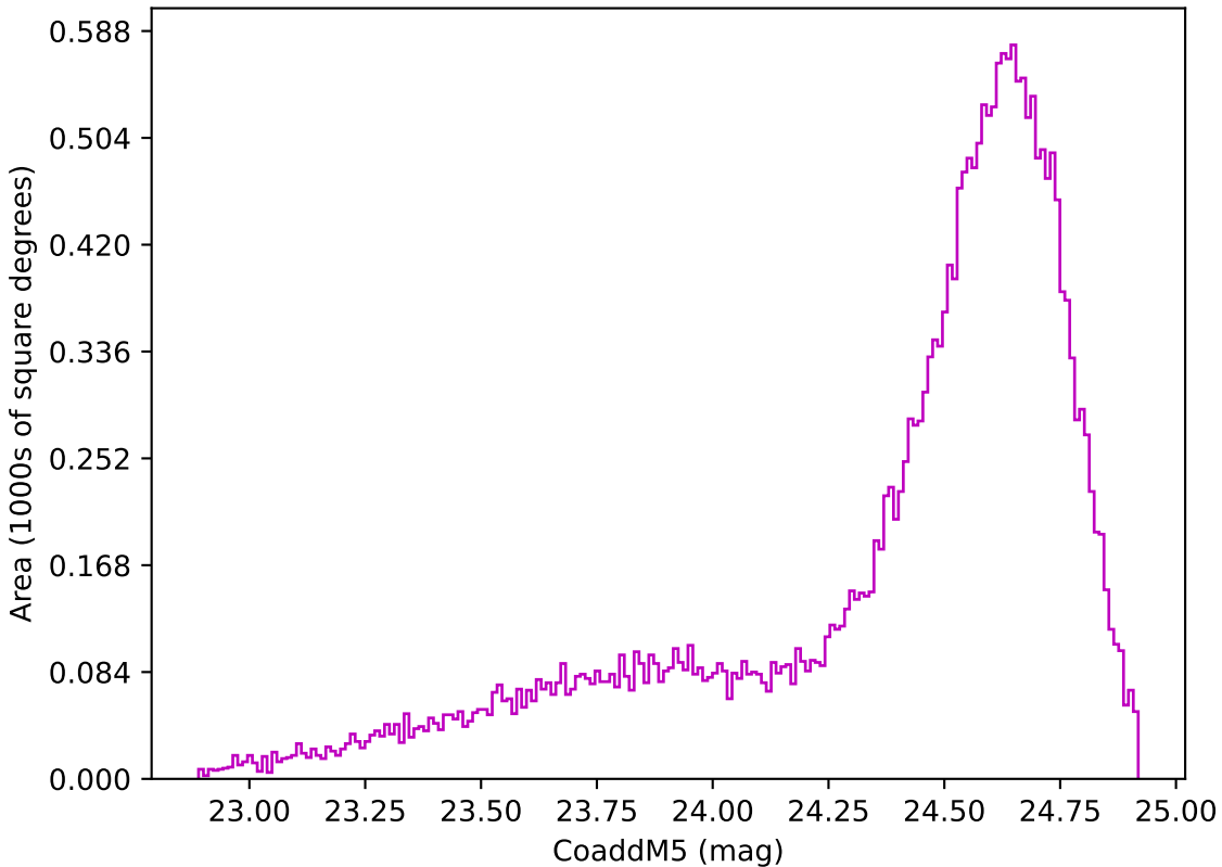
internal_u_expt45_nscale1.0v3.4_10yrs Yr 1 z band: CoaddM5
