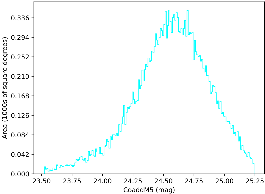
internal_u_expt45_nscale1.0v3.4_10yrs Yr 1 u band: CoaddM5
