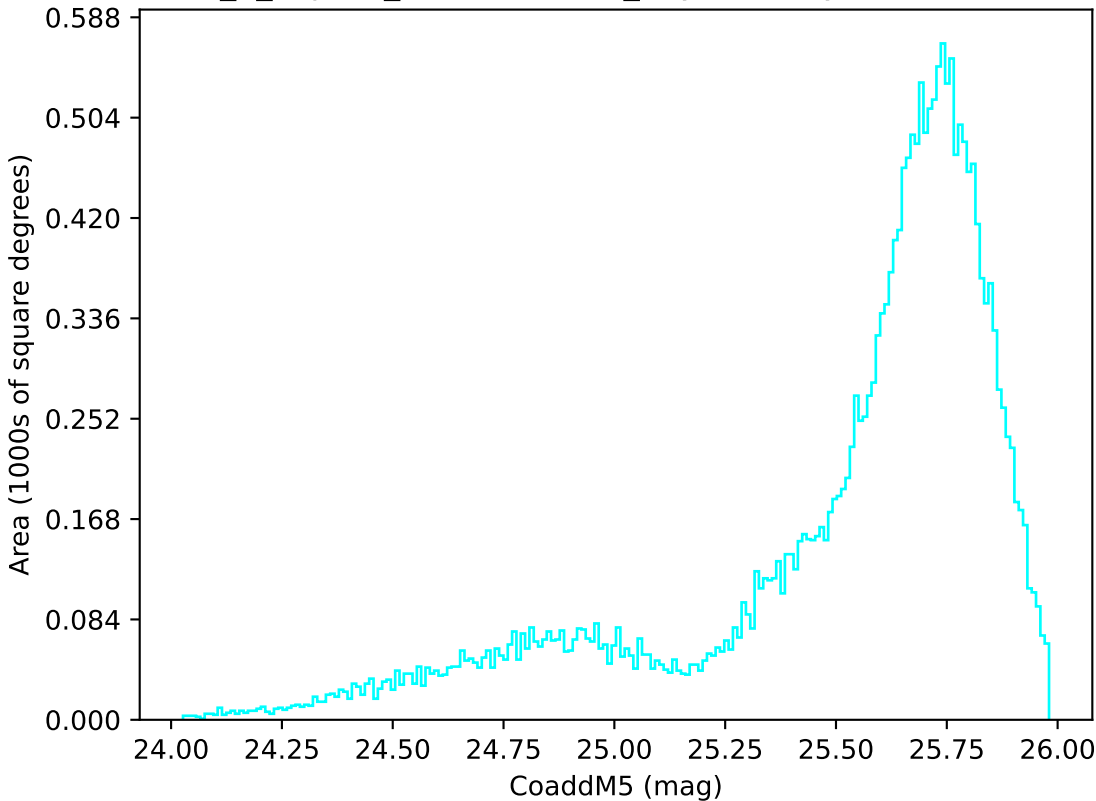
internal_u_expt45_nscale1.0v3.4_10yrs All sky u band: CoaddM5
