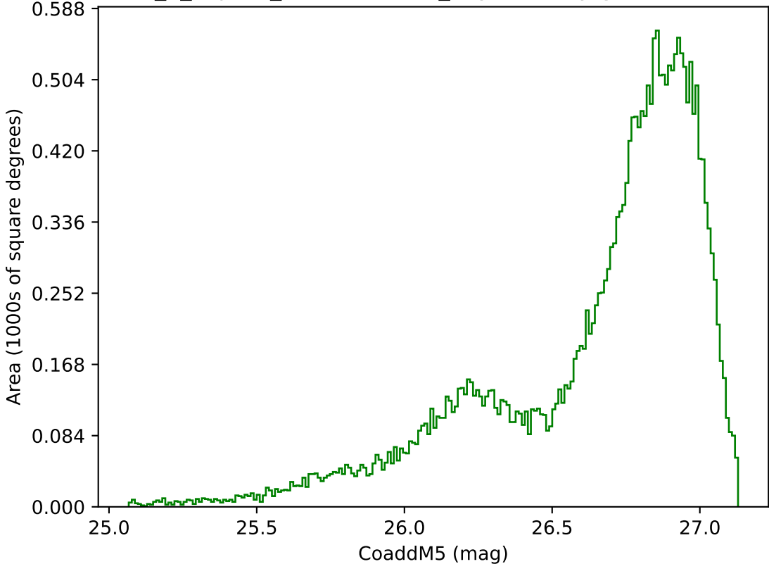
internal_u_expt45_nscale1.0v3.4_10yrs All sky g band: CoaddM5
