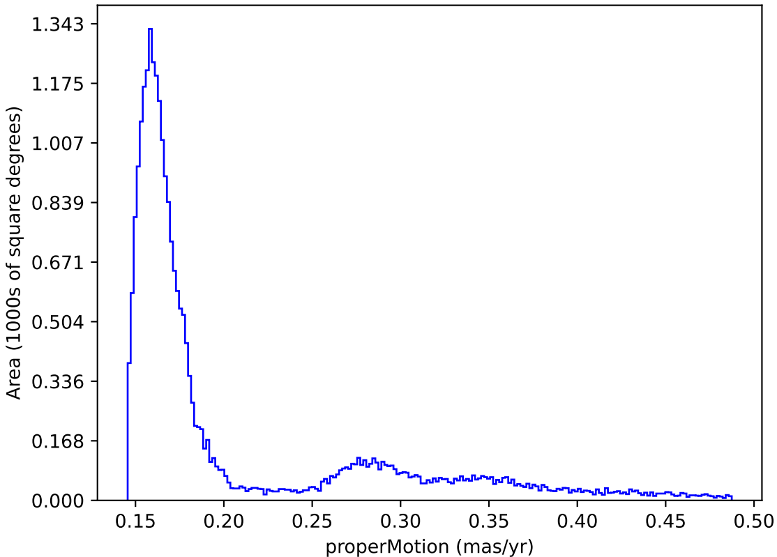
internal_u_expt45_nscale1.0v3.4_10yrs : properMotion
