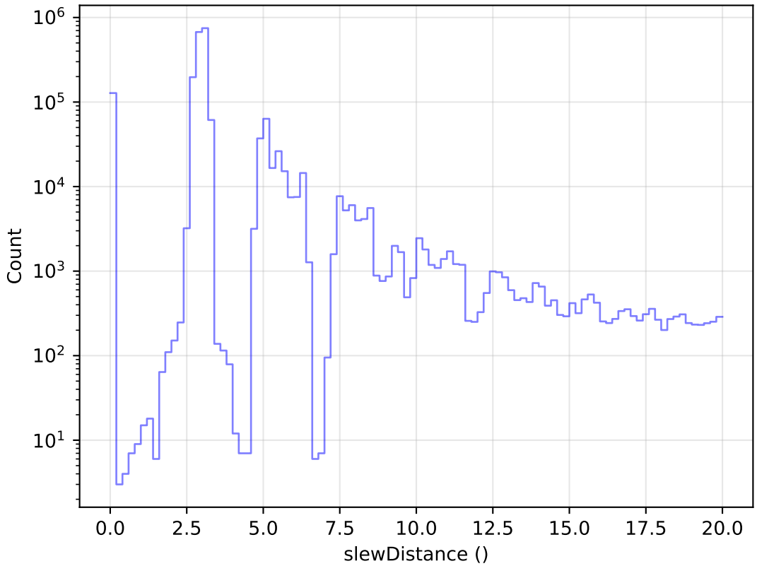
internal_u_expt45_nscale1.0v3.4_10yrs All visits: Zoom Slew Distance Histogram
