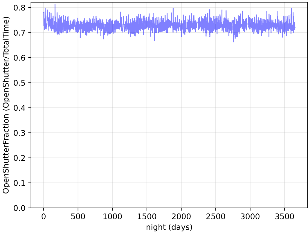
internal_u_expt45_nscale1.0v3.4_10yrs : OpenShutterFraction
