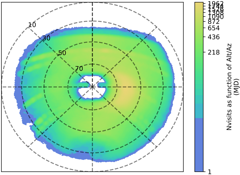
internal_u_expt45_nscale1.0v3.4_10yrs y: Nvisits as function of Alt/Az
