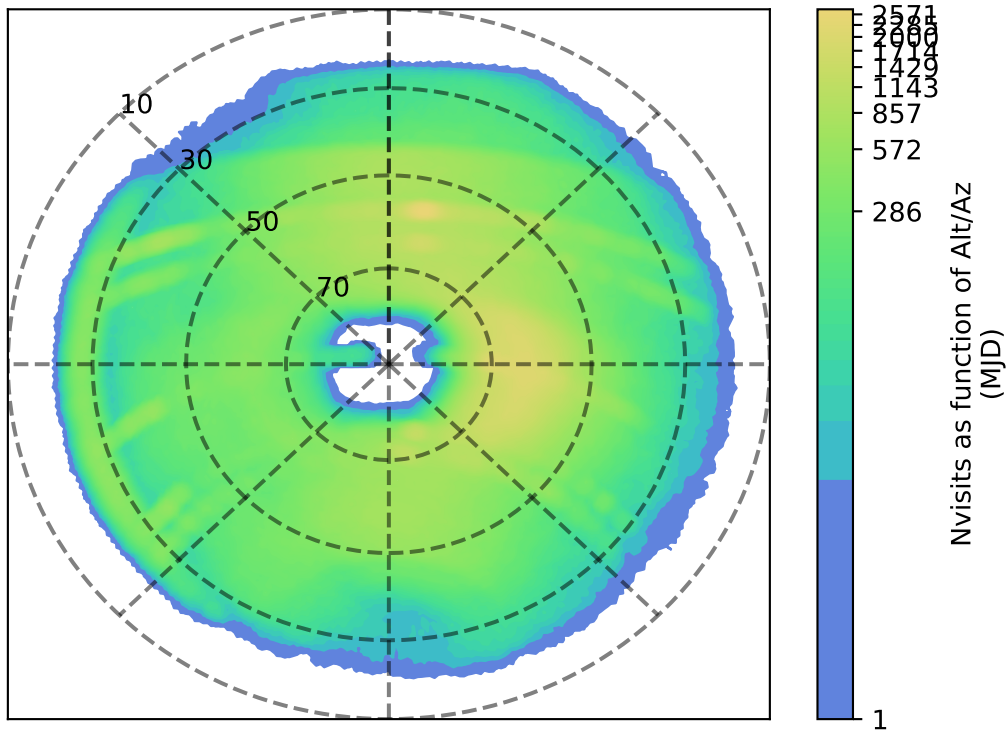
internal_u_expt45_nscale1.0v3.4_10yrs r: Nvisits as function of Alt/Az
