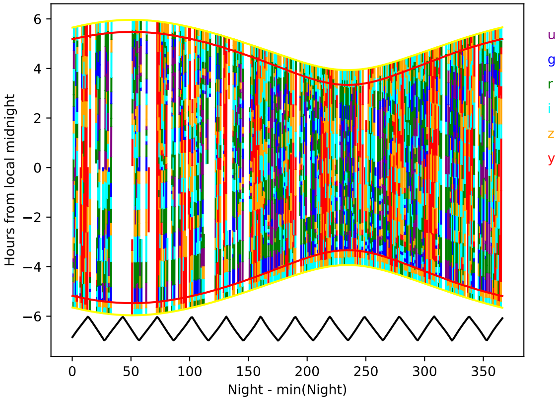
internal_u_expt45_nscale1.0v3.4_10yrs year 8-9: Hourglass
