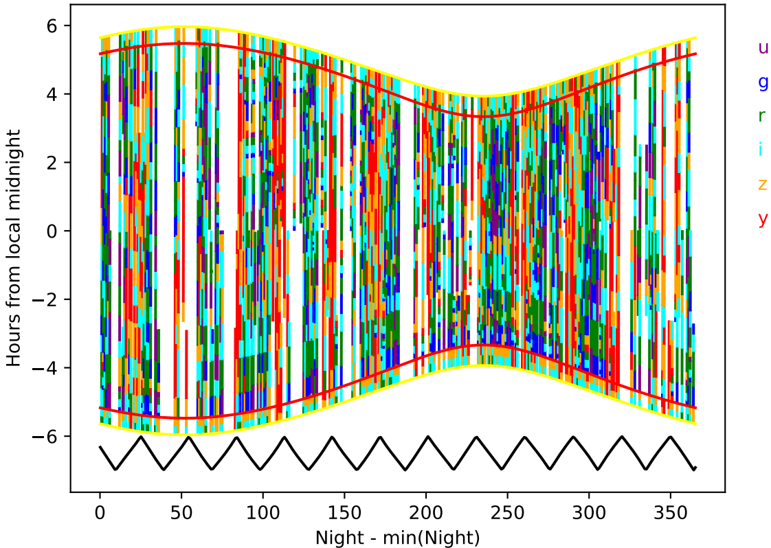
internal_u_expt45_nscale1.0v3.4_10yrs year 7-8: Hourglass
