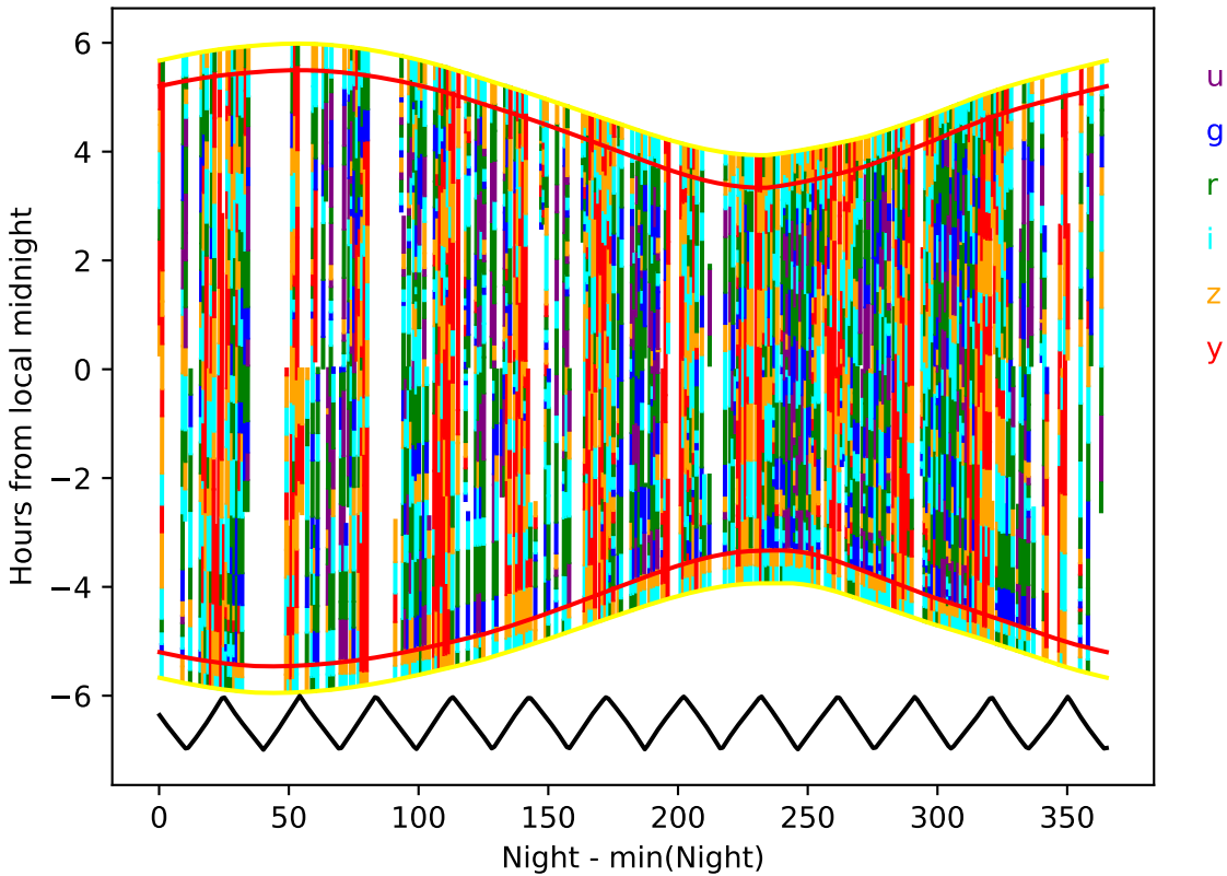
internal_u_expt45_nscale1.0v3.4_10yrs year 4-5: Hourglass
