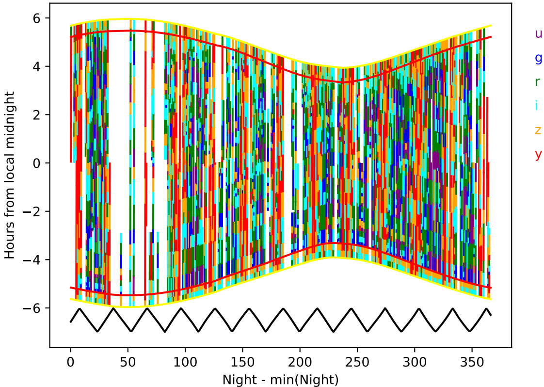
internal_u_expt45_nscale1.0v3.4_10yrs year 3-4: Hourglass
