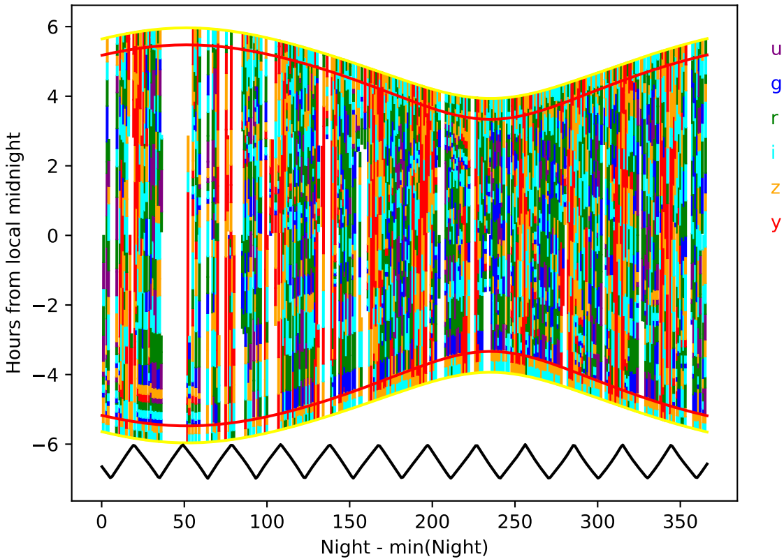
internal_u_expt45_nscale1.0v3.4_10yrs year 2-3: Hourglass
