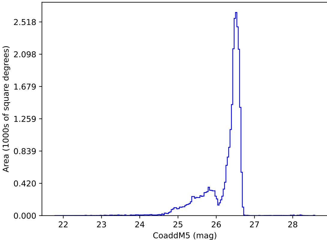
internal_u_expt45_nscale1.0v3.4_10yrs i: CoaddM5
