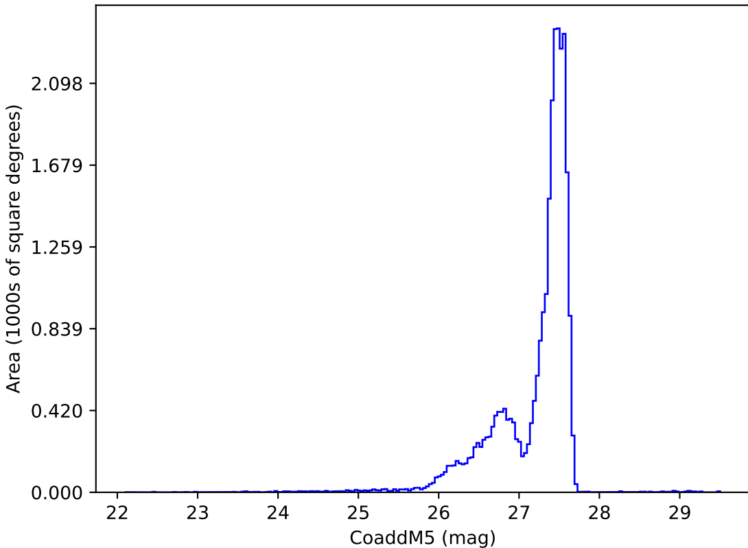
internal_u_expt45_nscale1.0v3.4_10yrs : CoaddM5
