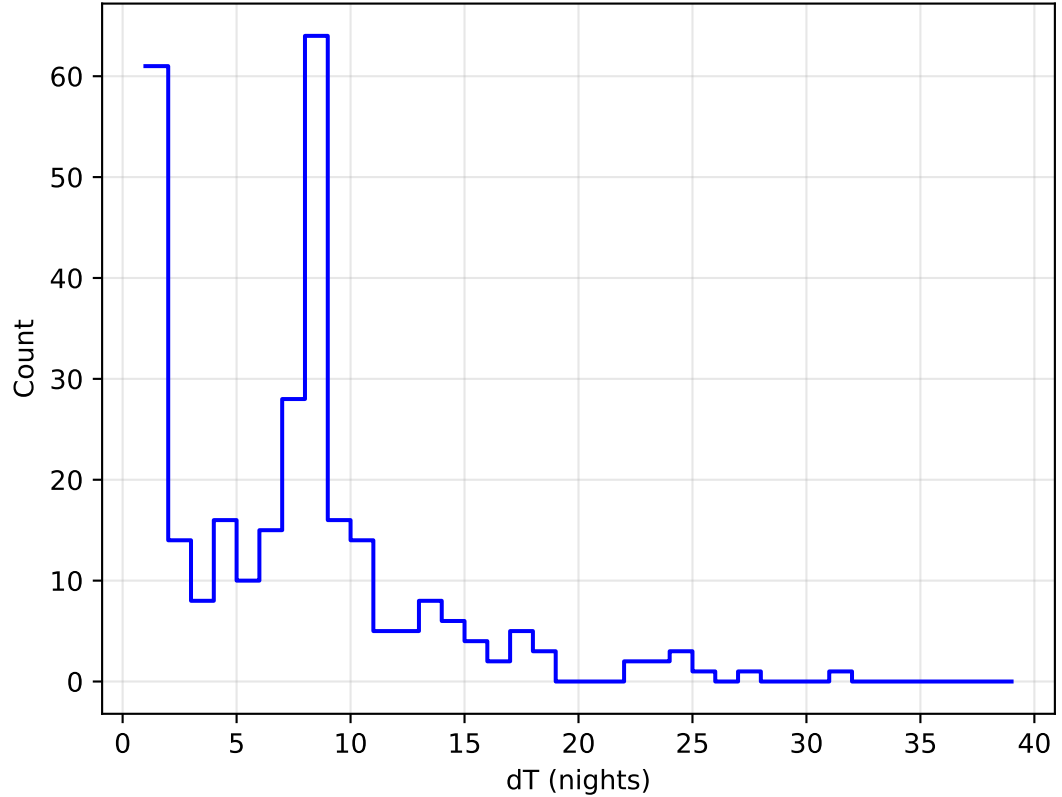
internal_u_expt45_nscale1.0v3.4_10yrs all bands: DD:XMM_LSS Delta Nights Histogram
