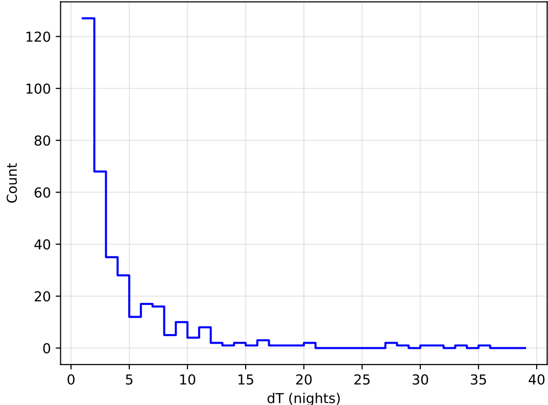
internal_u_expt45_nscale1.0v3.4_10yrs all bands: DD:WFD Delta Nights Histogram
