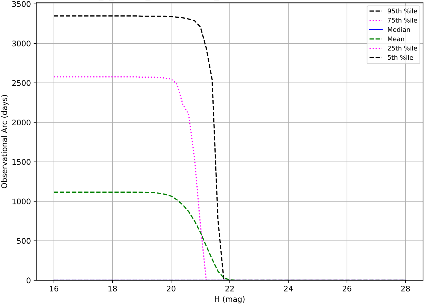
internal_u_expt45_nscale0.9v3.4_10yrs: Observational Arc Length Vatra
