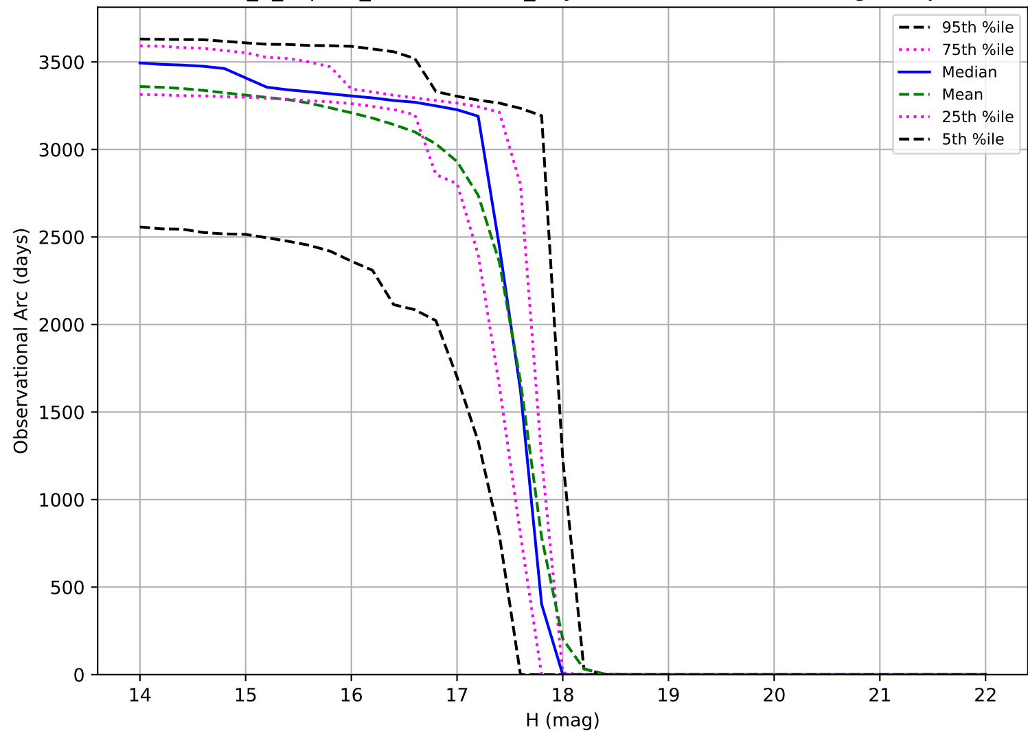
internal_u_expt45_nscale0.9v3.4_10yrs: Observational Arc Length Trojan
