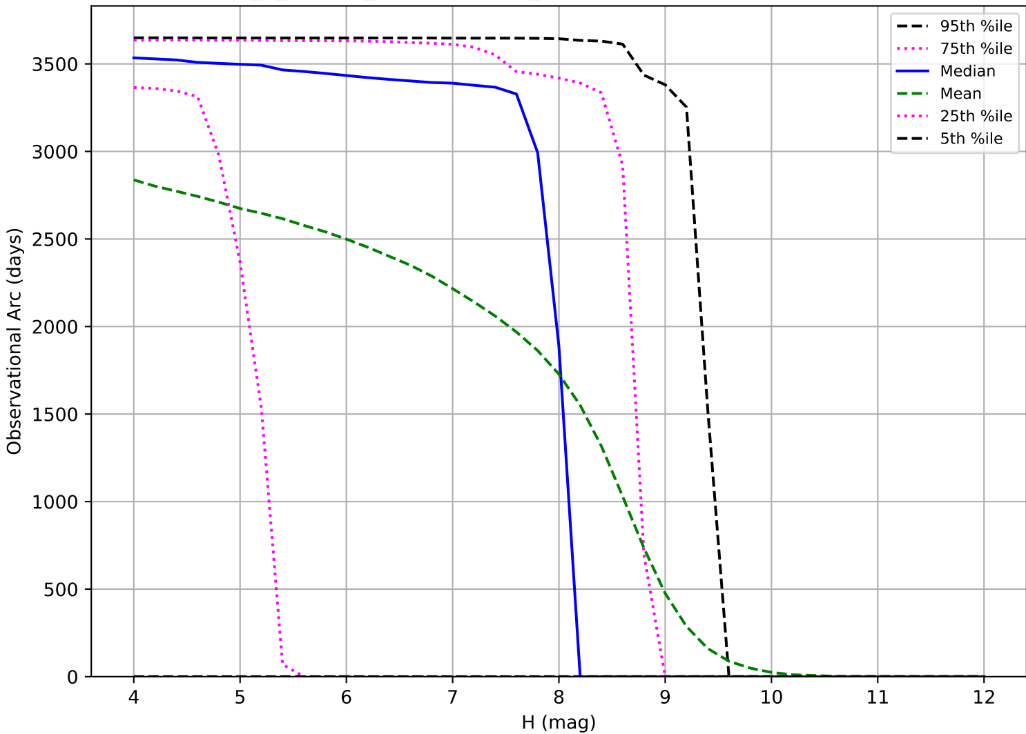
internal_u_expt45_nscale0.9v3.4_10yrs: Observational Arc Length TNO
