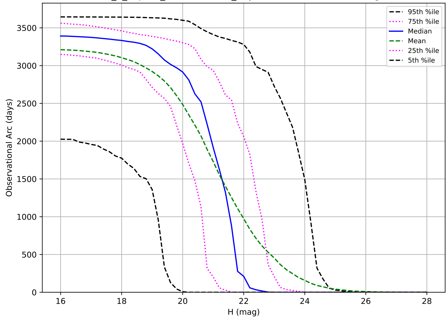
internal_u_expt45_nscale0.9v3.4_10yrs: Observational Arc Length PHA
